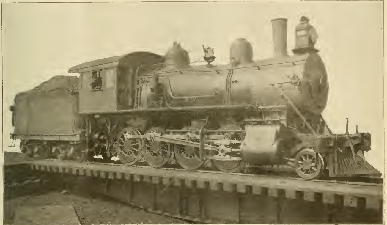
NORFOLK & WESTERN CONSOLIDATION—CLASS W.
